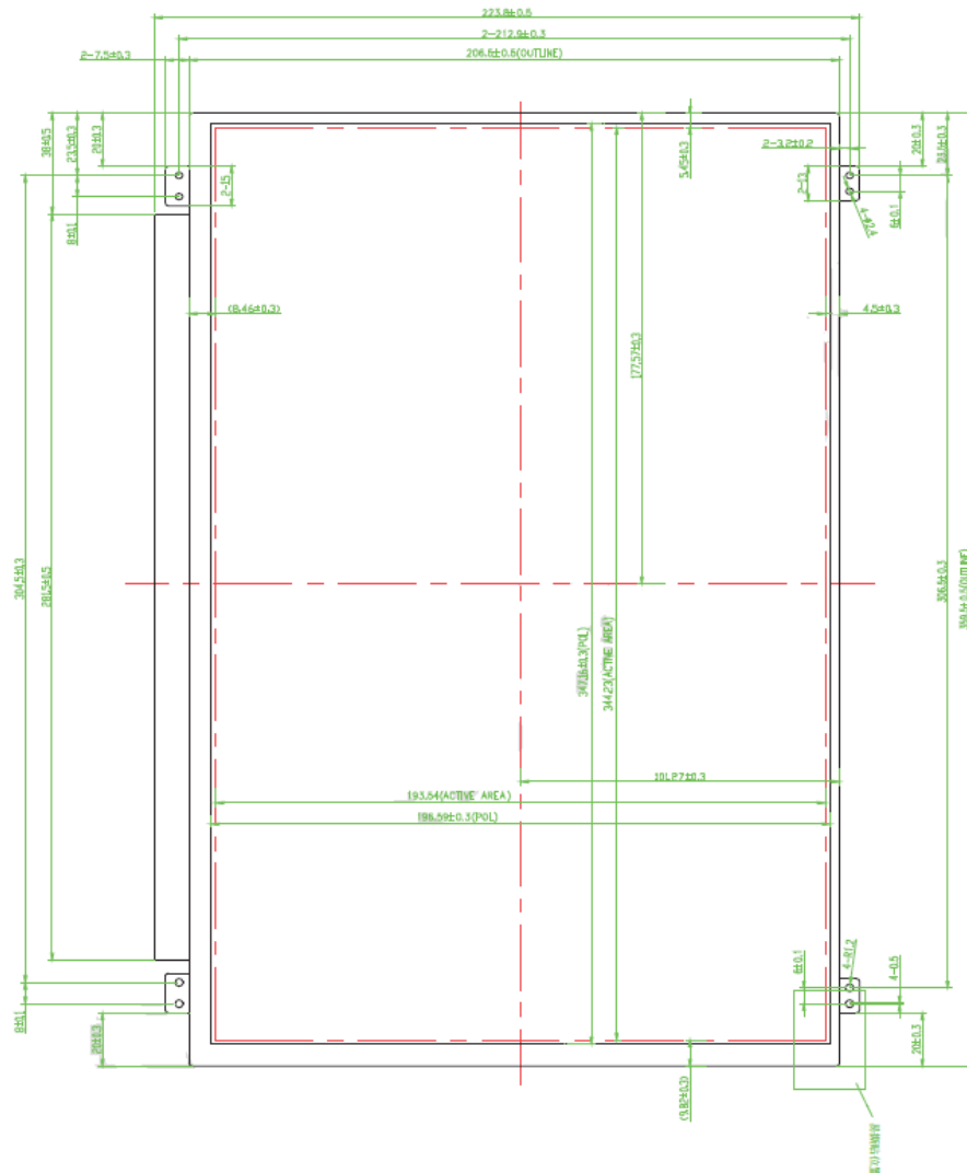
TFT-LCD Module Outline Dimension (Front View)
