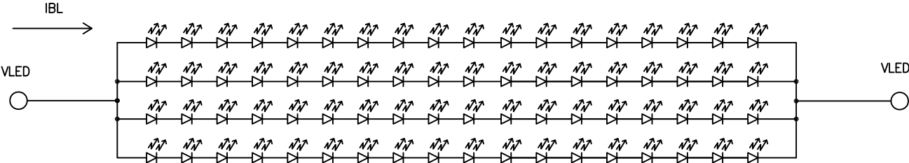
LED CIRCUIT
