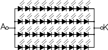
Backlight LED Circuit
