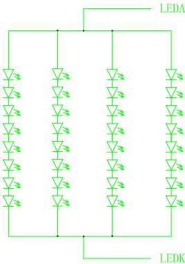
LED CIRCUIT
